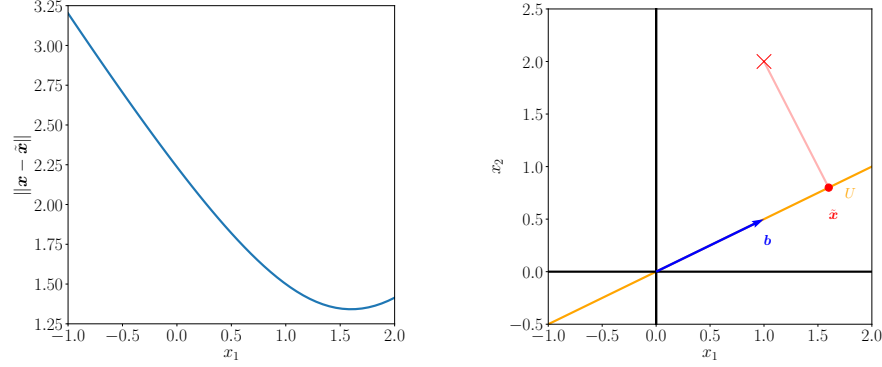
Figure 10.8 Optimal projection of a vector \mathbf{x} \in \mathbb{R}^2 onto a one-dimensional subspace (continuation from Figure 10.7). (a) Distances \|\mathbf{x} - \tilde{\mathbf{x}}\| for some \tilde{\mathbf{x}} \in U . (b) Orthogonal projection and optimal coordinates.
