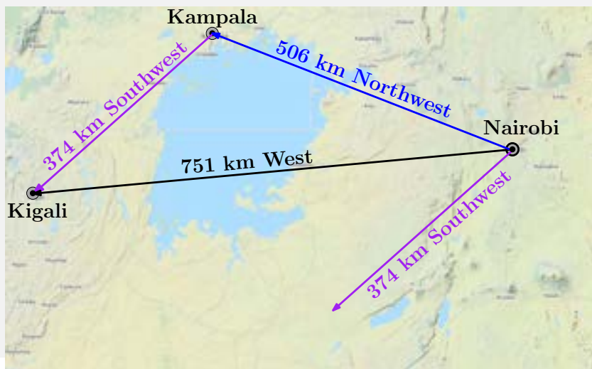
Figure 2.7 Geographic example (with crude approximations to cardinal directions) of linearly dependent vectors in a two-dimensional space (plane).
